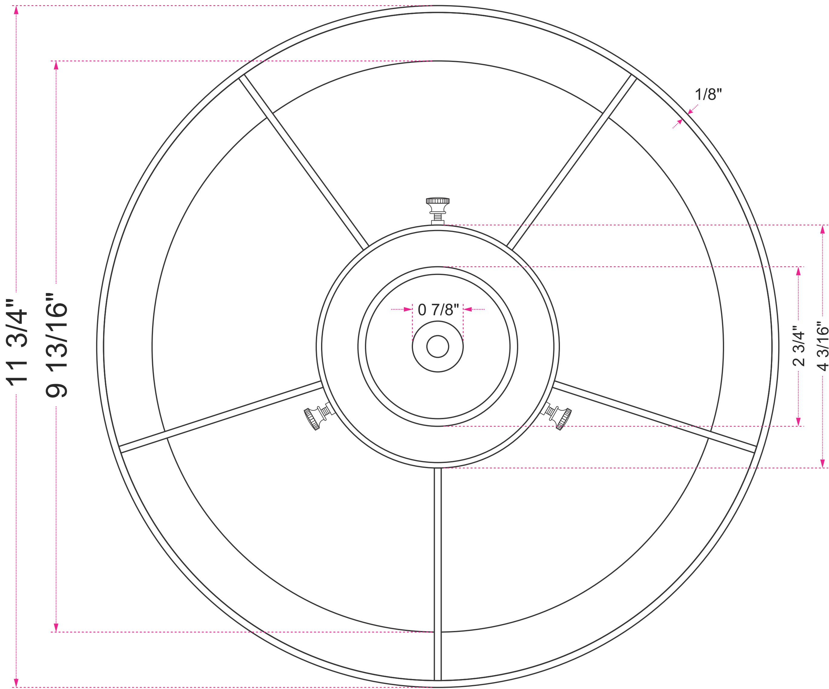
Front View
