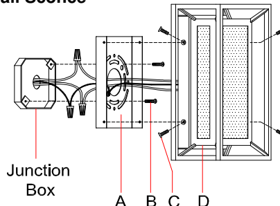
Fig. 1 Wall Sconce
