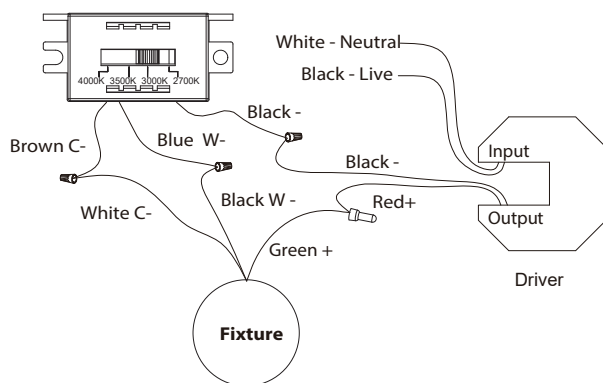
Fig.3 Driver Wires
