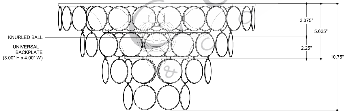
FRONT VIEW
